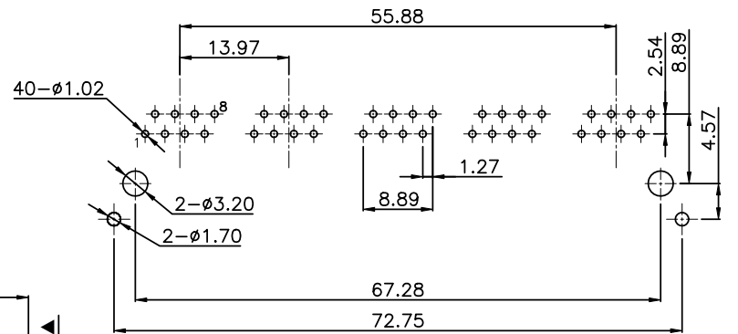
RECOMMENDED P.C.B LAYOUT TOP VIEW (COMPONENT SIDE DIM'±0.05)
