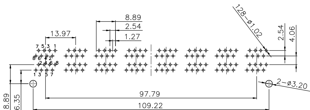
RECOMMENDED P.C.B LAYOUT TOP VIEW (COMPONENT SIDE DIM'±0.05)
