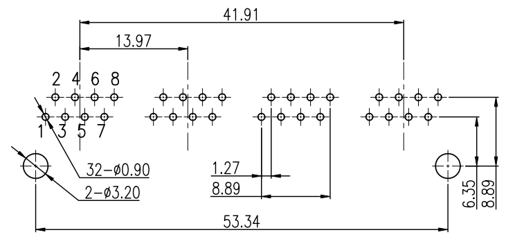
RECOMMENDED P.C.B LAYOUT TOP VIEW (COMPONENT SIDE TOLERANCE±0.05)
