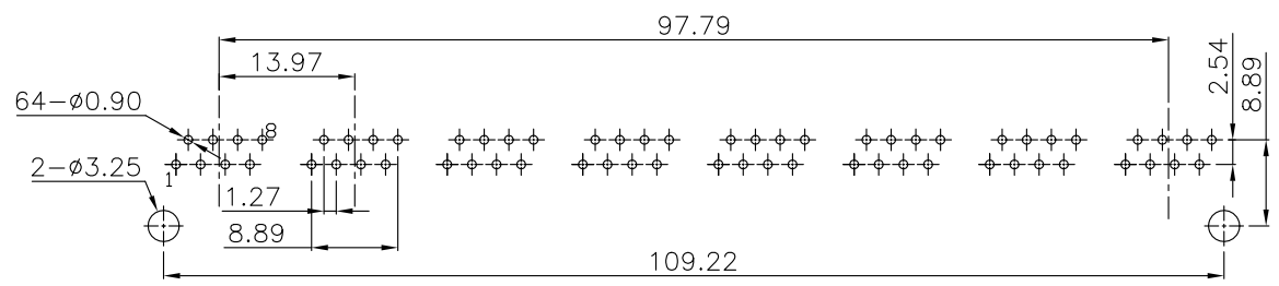
RECOMMENDED P.C.B LAYOUT TOP VIEW (COMPONENT SIDE TOLERANCE ±0.05)
