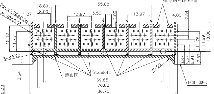
RECOMMENDED P. C. B LAYOUT TOP VIEW (Component side tolerance ±0.05 THICKNESS=1.6mm)
