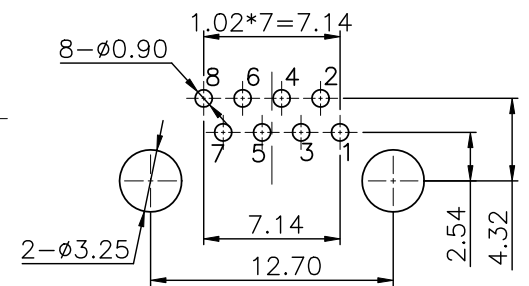
RECOMMENDED P.C.B LAYOUT TOP VIEW T=1.0~1.6(COMPONENT SIDE TOLERANCE±0.05)
