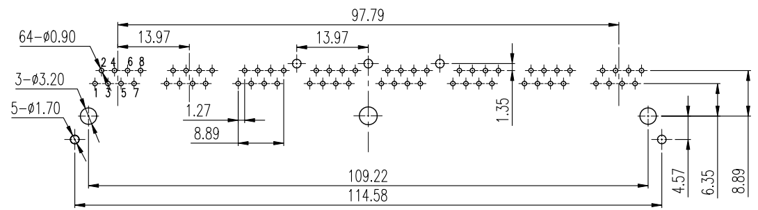
RECOMMENDED P. C. B LAYOUT TOP VIEW (COMPONENT SIDE DIM ±0.05)
