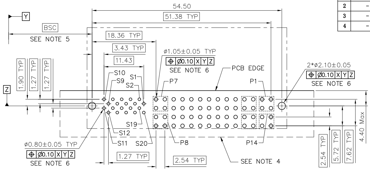
RECOMMENDED PCB LAYOUT TOLERANCE: ±0.05mm
