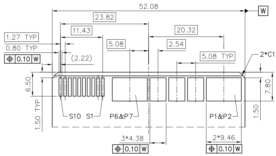
REFERENCE MATING CARD TOLERANCE: ±0.05mm
