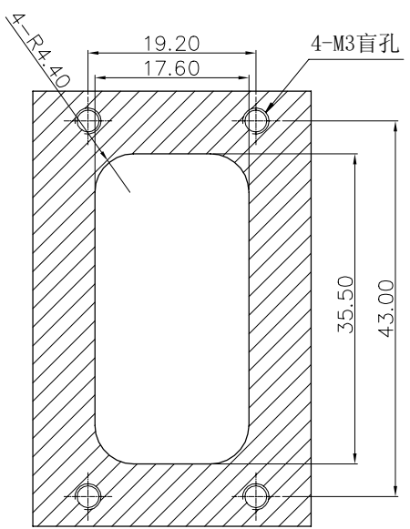
Recommend panel cutout
